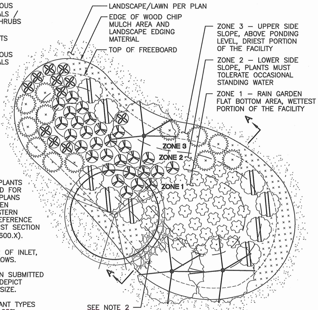
PLAN NTS
